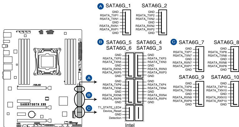
SABERTOOTH X99 Intel® SATA 6 Gb/s connectors
