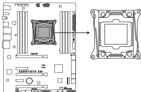
SABERTOOTH X99 CPU LGA2011-v3 Socket
