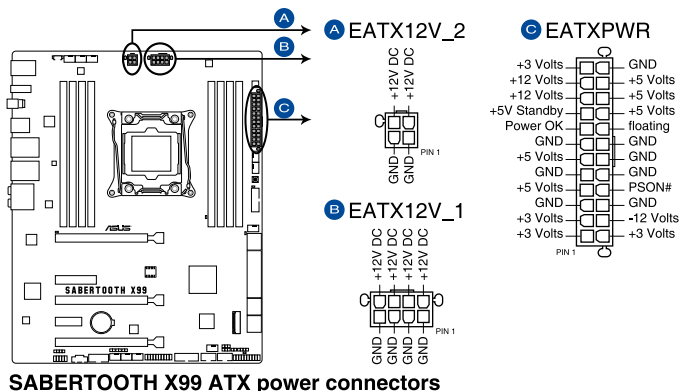
SABERTOOTH X99 ATX power connectors
