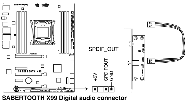
SABERTOOTH X99 Digital audio connector
