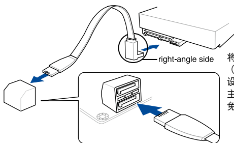
SABERTOOTH X99 Intel® SATA 6 Gb/s connectors
