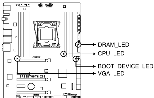
SABERTOOTH X99 CPU/ DRAM/ BOOT_DEVICE/ VGA LED
