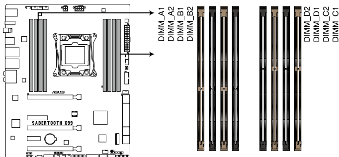
SABERTOOTH X99 288-pin DDR4 DIMM socket
